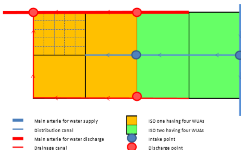
Figure 4: Schematic overview of intake points and discharge points for irrigated areas per ISO [8]
