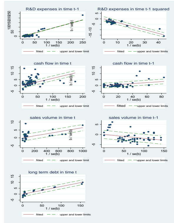
Figure 2: Galbraith plots
