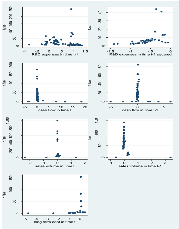
Figure 1: Funnel plots
